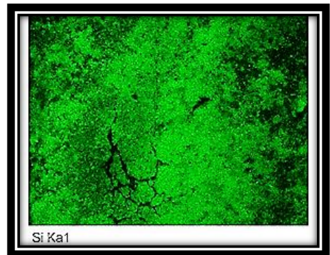
PED® image of silica scale
